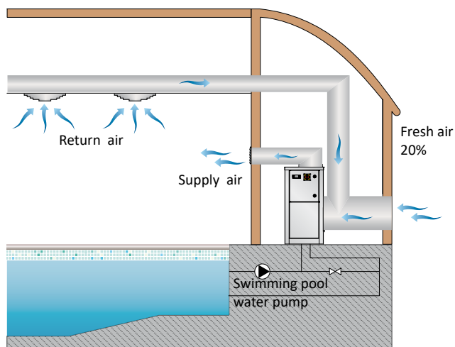
Plant scheme
